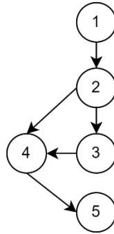
Gambar 7.6 Flow Graph Method broadcast()
