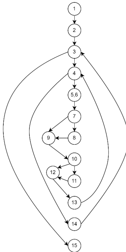
Gambar 7.1 Flow Graph Method cariPsikolog()
