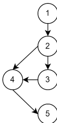
Gambar 7.4 Flow Graph Method cari_psikolog()
