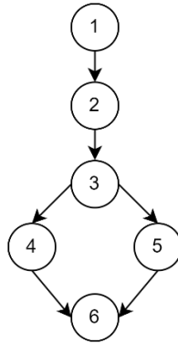
Gambar 7.3 Flow Graph Method buatMessage()
