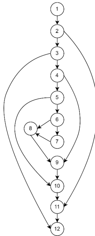
Gambar 7.5 Flow Graph Method tambah()
